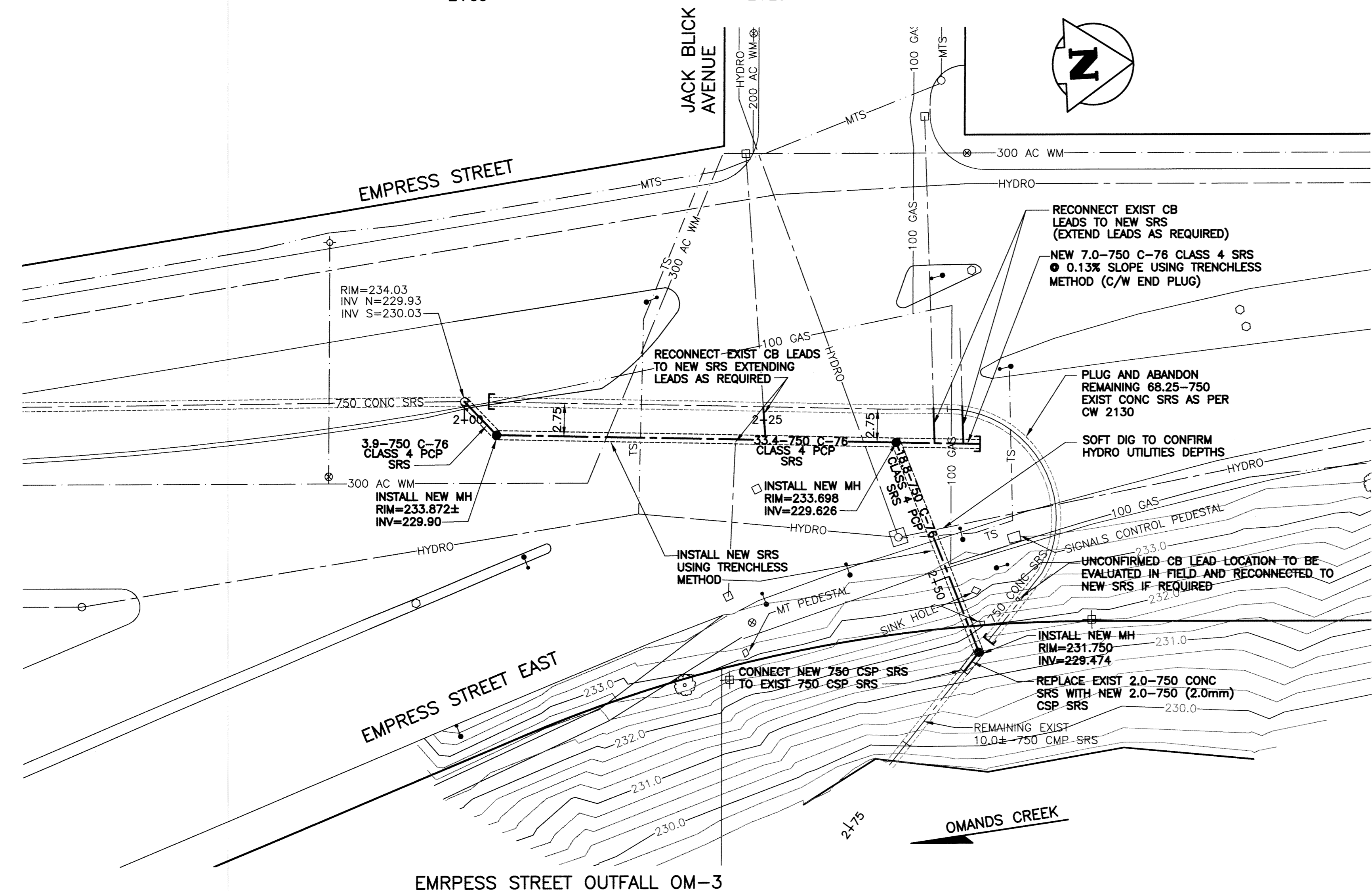
EMRESS STREET OUTFALL OM-3
